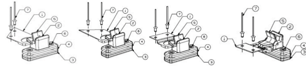
Latch for Sliding Window (4 pieces)
